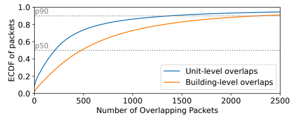
Figure 7: Distribution of unit-level and building-level overlaps over all packets.
