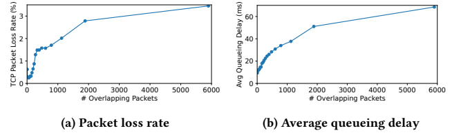
(a) Packet loss rate (b) Average queueing delay Figure 4: Correlation between the number of unit-level overlaps per packet and congestion metrics.
