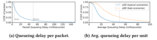
(a) Queueing delay per packet. (b) Avg. queueing delay per unit Figure 3: CCDF of access queueing delay.
