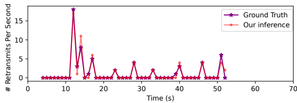
Figure 19: Our inference of TCP retransmits closely matches the ground truth.
