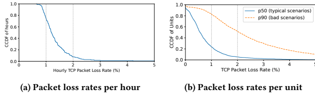
(a) Packet loss rates per hour (b) Packet loss rates per unit Figure 2: Access TCP packet loss rate across hours and units.
