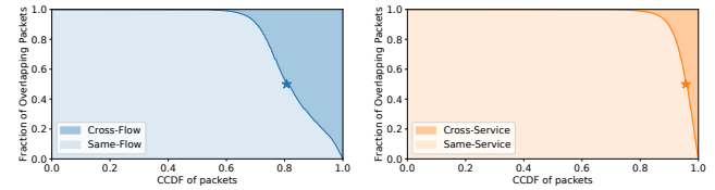
(a) Same-flow vs. cross-flow
